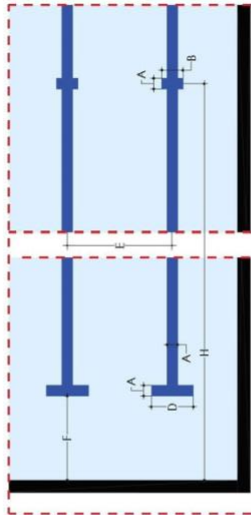
FIG. 4 PLAN LANE MARKINGS
